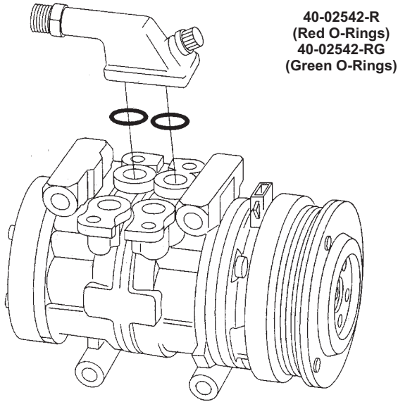
Ford, Special Compressor O-Rings with Oval Cross Section
