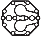
21-84600 YORK FULL SIZE COMPRESSOR HEAD GASKET 209 / 210
