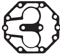
21-26005 YORK HEAD GASKET - EARLY MODEL
