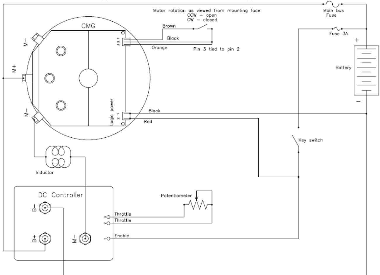
Typical Low Side PWM DC Controller Application
